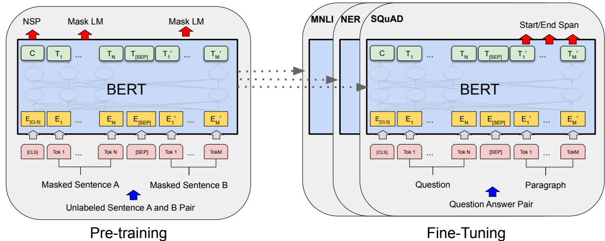
Figure 7: Overall pretraining and fine-tuning for BERT. Reproduced from BERT paper [Devlin et al., 2019]
