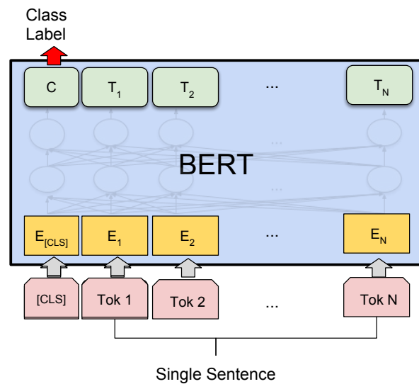
Figure 8: Fine-tuning BERT for single sentence classification by adding a layer on top of the contextualized [CLS] token representation. Reproduced from BERT paper [Devlin et al., 2019]
