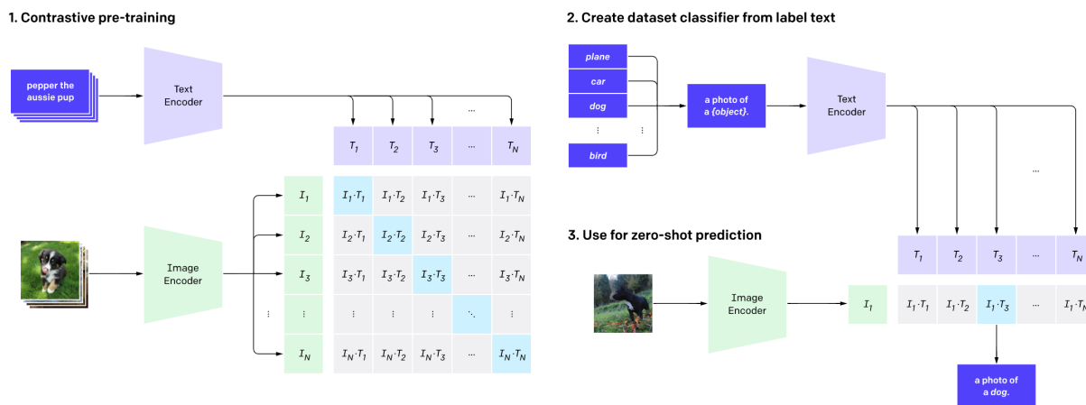
Figure 9: 1. Contrastive pre-training task that predicts the caption that corresponds to an image out of many possible captions. 2. At test time, each class is converted to a caption. This is used with 3. as a zero-shot classifier for a new image that predicts the best (image, caption) pair. Figure taken from [Radford et al., 2021a]
