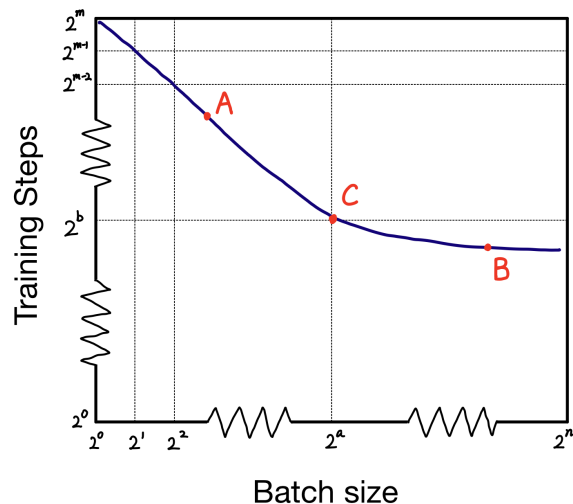
Figure 1: A cartoon illustration of the typical relationship between training steps and the batch size for reaching a certain validation loss (based on Shallue et al. [2018]). Learning rate and other related hyperparameters are tuned for each point on the curve.
