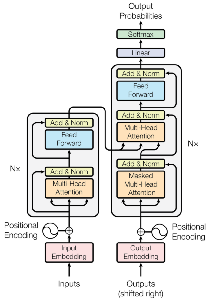
Figure 4: The transformer architecture. Vaswani et al. [2017]
