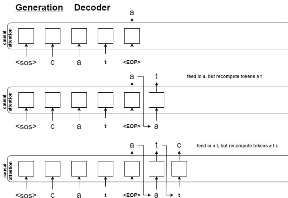
Figure 6: Translating a text using the decoder-only NMT model.
