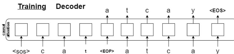
Figure 5: Training the decoder-only NMT model.
